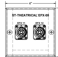
NEMA TYPE 1 BBX -4x4x4, PLATE 4x4 6 (ST-S-TE-2-08) SPEAKER - THEATRICAL EFFECTS SCALE: 1:1 (SURFACE MOUNTED, BEVELED, BLACK)
